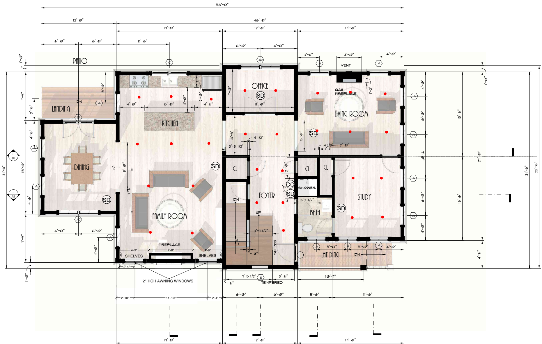
FIRST FLOOR
